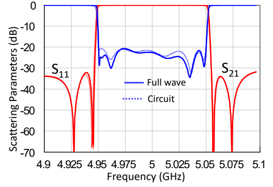
Fig. 7. Response of the dimensioned path filter with full wave analysis (solid lines). For comparison, the response of the equivalent circuit with ideal couplings (Fig. 5a) is also reported (dashed lines).
