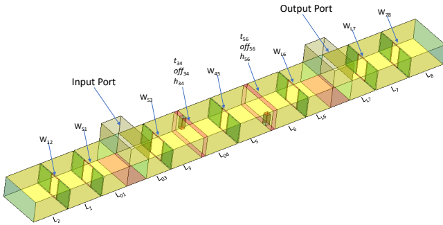
Fig. 6. Drawing of the novel path filter with the relevant dimensions (all irises have the same thickness tW=1\text{mm} ).
