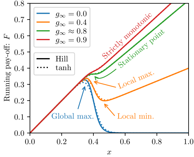
Figure 14: The running pay-off F(x) = g(x)x for different parametrisations of g(x) . Solid curves show the Hill form (29d) while dashed curves show the (nearly identical) hyperbolic tangent form (136) sharing the same parameter values: g_0 = 1 , K = 0.4 , n = 20 . When g_\infty = 0 we observe the global maximum. When g_\infty \in (0, g_c) , where g_c \approx 0.8186 is such that 4cn = (n-1)^2 , there are two roots of f corresponding to the local maximum and the local minimum. When g_\infty = g_c there is a unique double root of f corresponding to a stationary point. For g_\infty > g_c the F curve is strictly monotonic.
