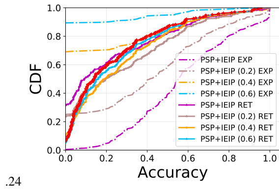
Figure 29: IEIP
