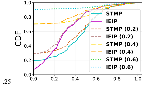
Figure 13: Precision
