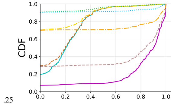
Figure 14: Recall
