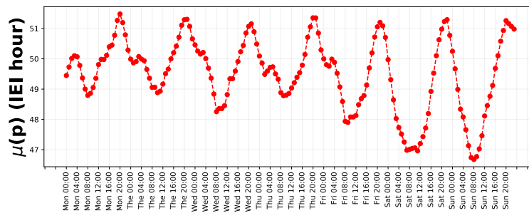
Figure 36: IEI mean.
