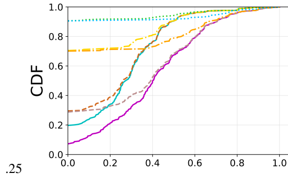
Figure 15: F1-Score
