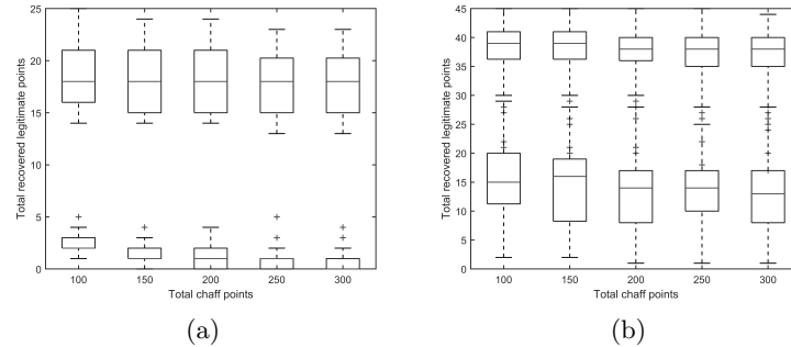
Fig. 2: The distribution of recovered legitimate points for both valid and invalid claims for the different number of chaff points. Figure 2a for Touchalytics based BAVault and Figure 2b for DAC based BAVault.
