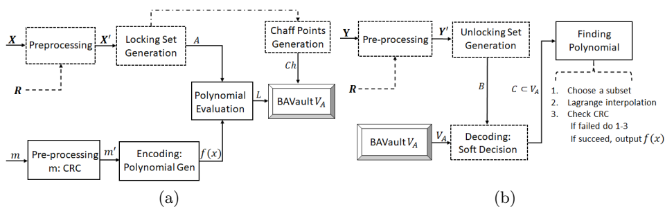
Fig. 1: Block diagram of BAVault (a) locking and, (b) unlocking.
