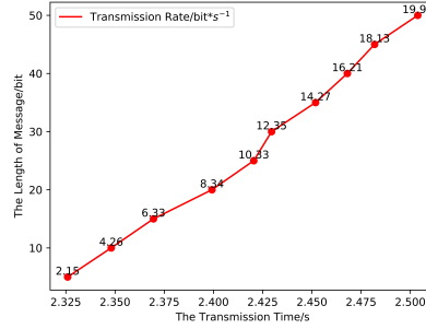
Fig. 5. The Encrypt Rate in CCBRSN
