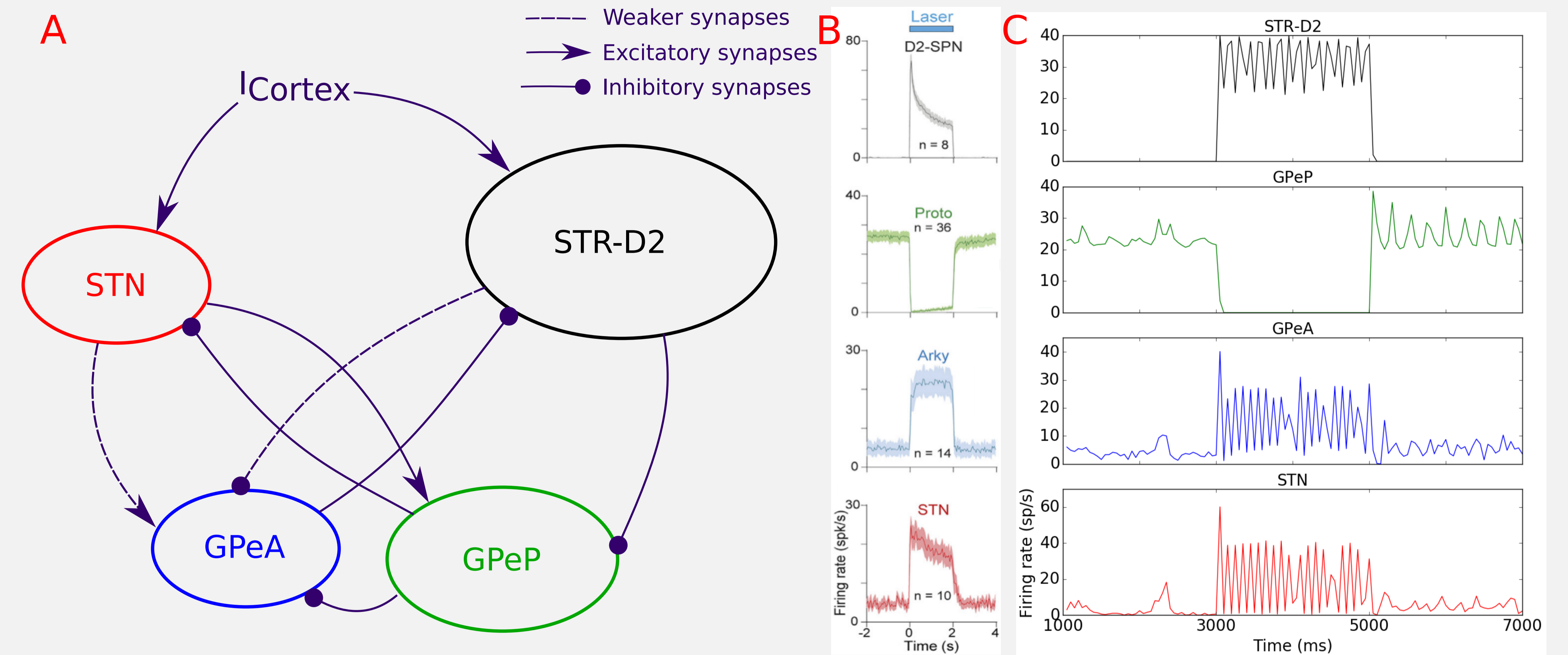
Figure: A Basal ganglia model STN-GPeA-GPeP-STR(D2) with the connectivity. B, C Comparing biological data with simulated data. STN-GPeA-GPeP-STR(D2) firing rate between 1-7s (simulated data) and between (-2)-4s (biological data). STR-D2 activated with a stimulation between 3-5s (simulated data) and between 0-2s (biological data). GPeP and GPeA react oppositely. B Biological data reproduced from [2] with the courtesy of the authors. C Simulated data. Firing rate during stimulation for STN: 20.0 +/- 3.8 Hz, GPeA: 15.9 +/- 3.2 Hz, GPeP: 0.1 +/- 0.4 Hz, STR-D2: 32.3 +/- 0.8Hz.
