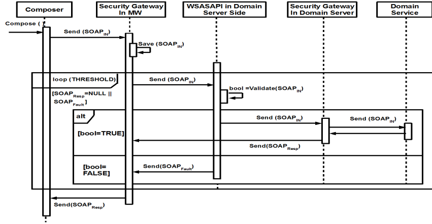
Fig. 3. Securing message communication from WSAS attack
