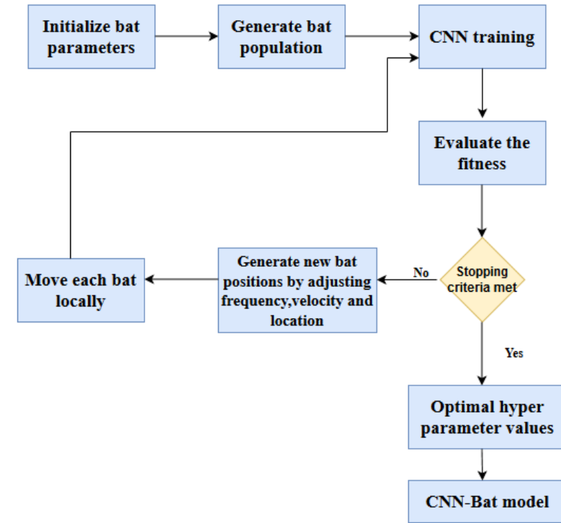
Fig. 3. Process flow of Bat-CNN
