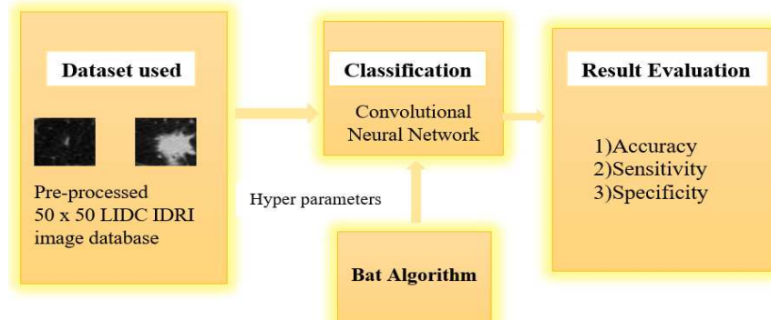
Fig. 1. Proposed Methodology
