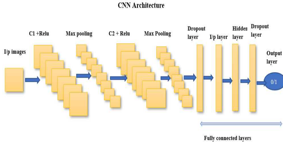
Fig. 2. CNN Architecture
