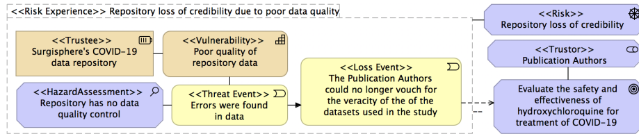
Fig. 14: Risk Experience
