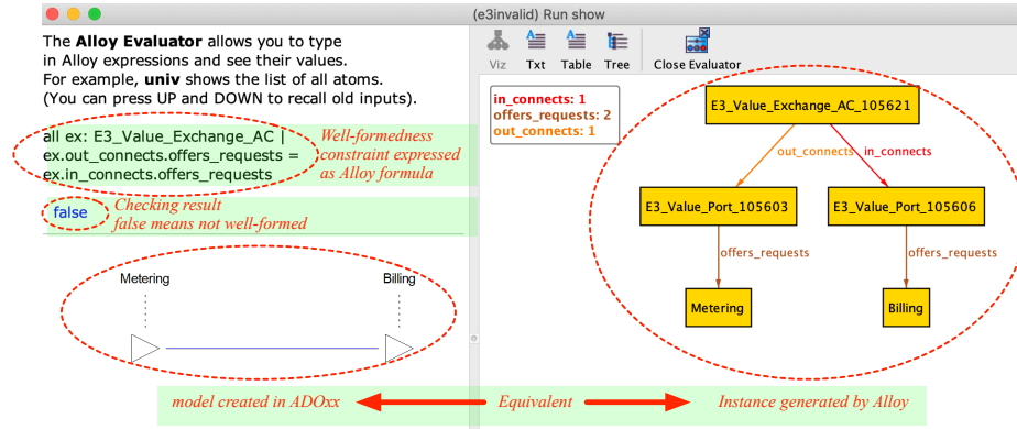
(b) Model in Fig. 4b is not well-formed
