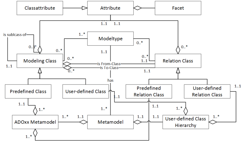
Fig. 1: An excerpt of the meta meta model as used by ADOxx Development Toolkit [9]
