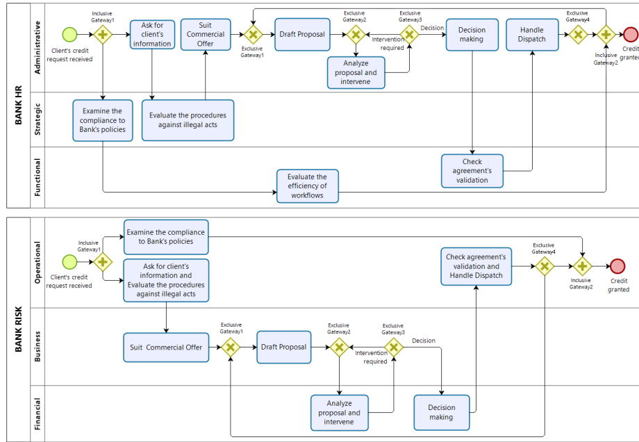
Fig. 3. BPMN process views of the Bank Credit Granting process, designed by HR (top) and Risk (bottom) departments.
