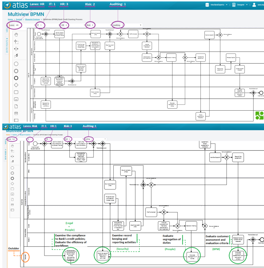
Fig. 4. Screen of the Atlas tool after the generation of HR (top) and Risk (bottom) business process views at level 3 of detail.
