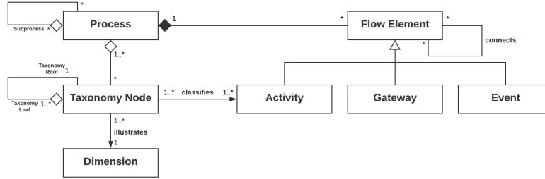
Fig. 2. UML class diagram of the Atlas tool’s process repository metamodel.
