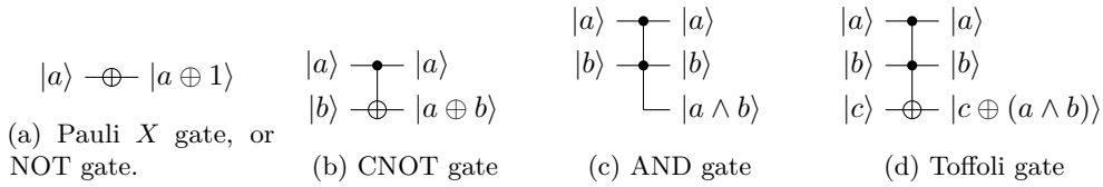
Figure 1: Quantum gates used in quantum implementations of classical circuits
