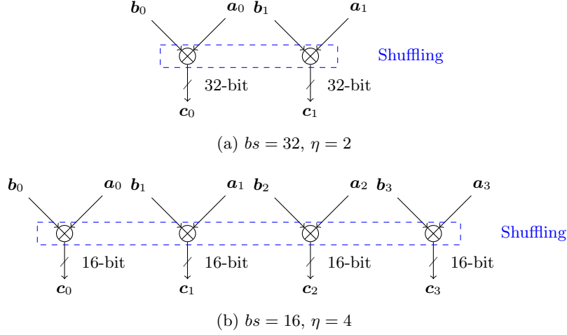
Fig. 8: Different options in the design space for \#AND=64 .
