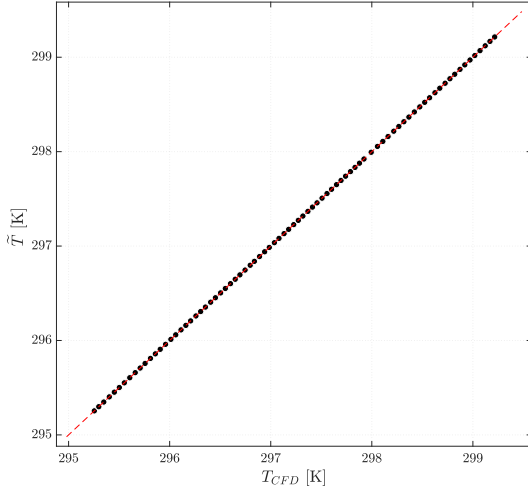
Figure 6. Comparison of surrogate model evaluations of temperature \tilde{T} with the CFD model for a given input \bar{R}^{(i)} . The red line represents the first bisector curve.
