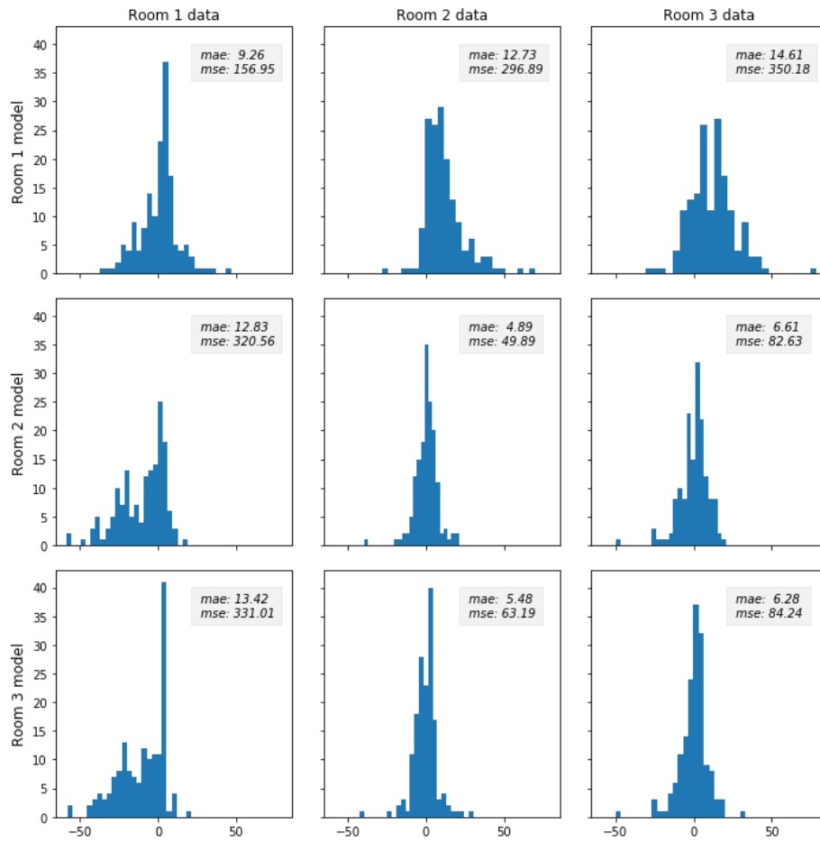
Fig. 6. Predicting space occupancy by self-trained model vs. transferred models. The histogram plot in each cell shows the distribution of errors for the occupancy counting task.
