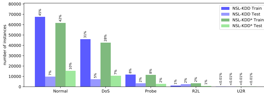
Fig. 1. The distribution of samples in the NSL-KDD dataset
