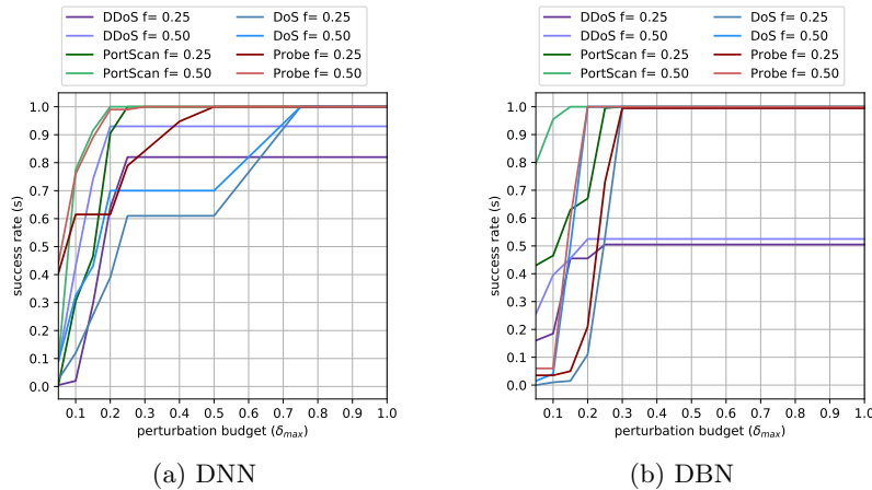
Fig. 4. The success rate of attacks against the DNN and DBN models for different values of \delta_{max} parameter
