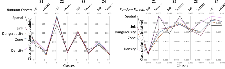
Fig. 8. Absolute (left) and relative (right) class confusions of the most promising models.
