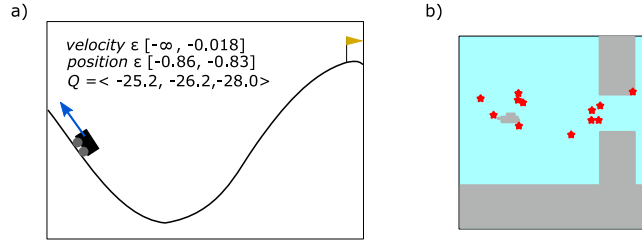
Fig. 5. Examples of a) rule extraction, and b) super-pixels extracted by the LMUTs in Liu et al. [37]. a) Extracted rules for the mountain Cart scenario. Values at the top are the range of velocity and position and a Q vector ( Q_{move\_left}, Q_{no\_push}, Q_{move\_right} ) representing the average Q-value). In this example, the cart is moving to the left to the top of the hill. The car should be pushed left ( Q_{move\_left} is highest) to prepare for the final rush to the target on the right side. b) Super-pixels for the Flappy Bird scenario, marked by red stars. This is the first of four sequential pictures where the focus lies on the location of the bird and obstacles (i.e., pipes). In later pictures the focus would shift towards the bird’s location and velocity.
