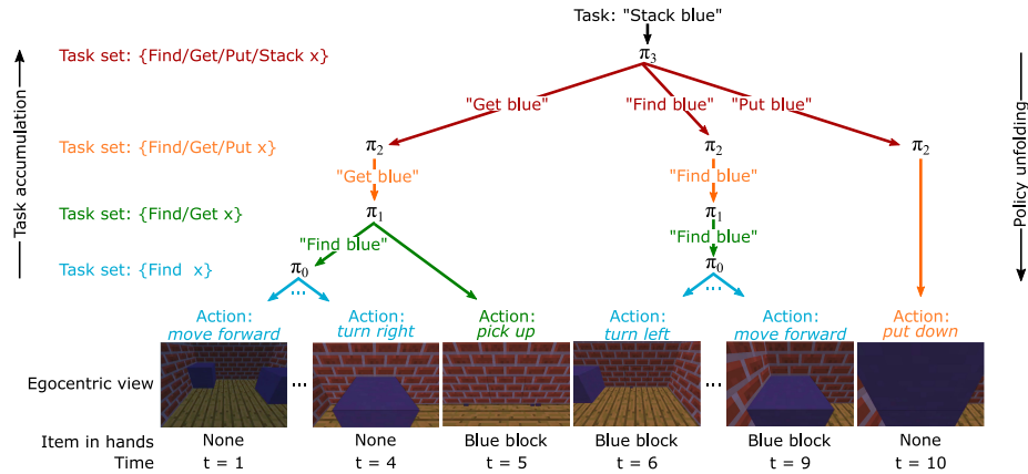
Fig. 4. Example for the mutli-level hierarchical policy for the task to stack two blue boxes on top of each other. The top-level policy ( \pi_3 , in red) encompasses the high-level plan ‘get blue’ \rightarrow ‘find blue’ \rightarrow ‘put blue’. Each step (i.e., arrow) either initiates another policy (marked by a different color) or directly executes an action. Adopted from Shu et al. [53] .
