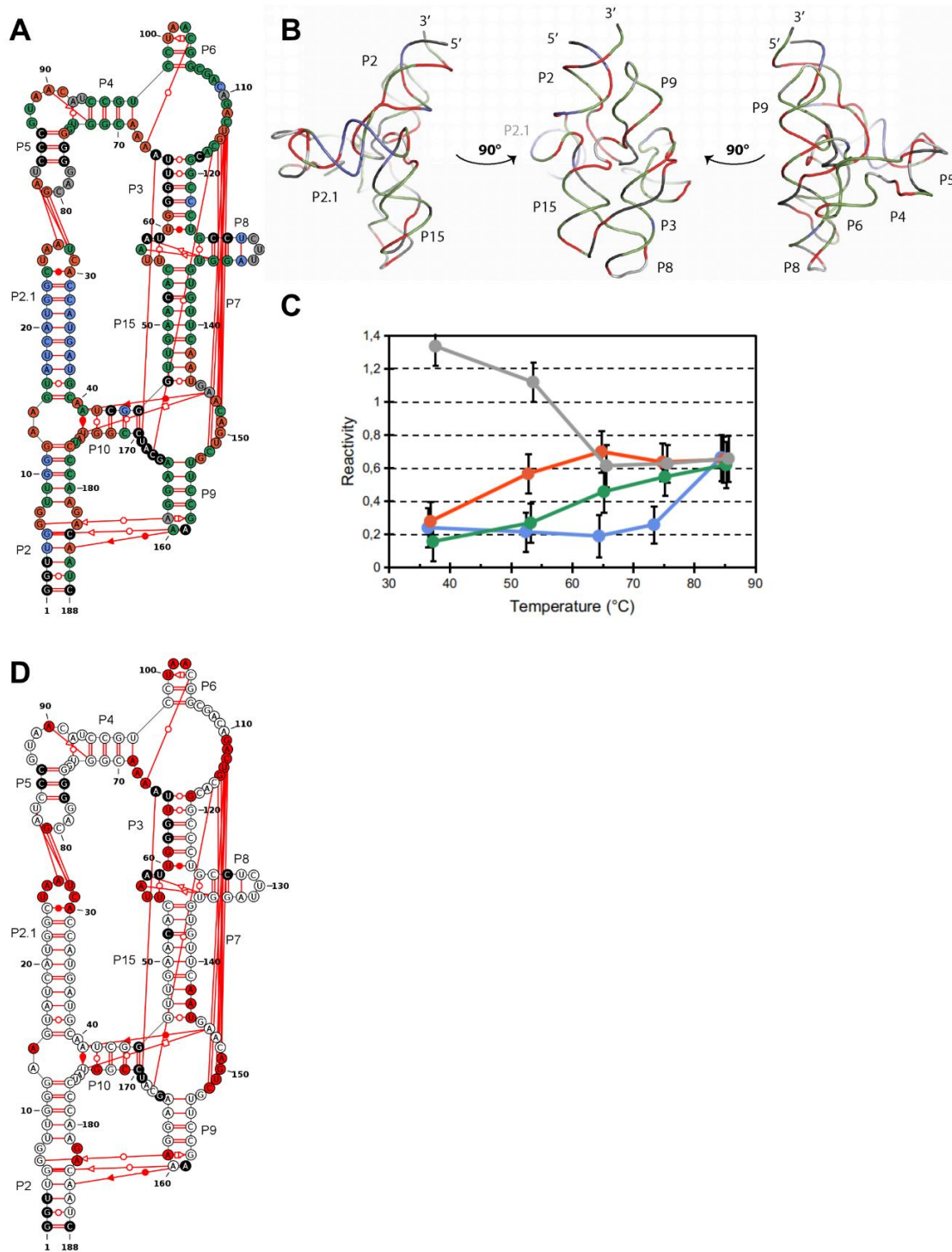
Figure 3. DiLCrz reactivity profiles at different temperatures. DiLCrz structure was probed with 1M7 at 37, 53, 65, 74 and 85 °C in 40mM HEPES pH 7.5, 500 mM KCl and 5 mM MgCl 2 . (A) Clustering of the nucleotides according to their reactivity change. KMeans clustering was performed on 1M7 reactivities. DiLCrz secondary structure coloring refers to the nucleotides' assigned clusters. (C) Previously reported DiLCrz X-ray structure (Meyer et al. 2014) colored according to the clustering. (B) Evolution of the average reactivity within each of the four clusters. Error bars refer to the reactivity mean absolute deviation within each cluster. Points are horizontally jittered for clarity. (D) Comparison of 1M7 reactivities between 37 and 53 °C. Significant reactivity differences are highlighted in red. The comparison was performed as described in Material and Methods. Nucleotides in black denote undetermined reactivity.
