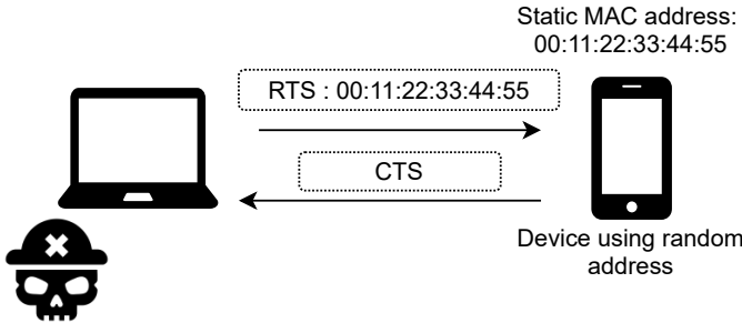
Fig. 3. RTS-CTS attack [20, sec 6.7] forcing a device using address randomization to reveal its presence. The attacker emits an RTS frame targeting the real MAC address of the victim; the victim will automatically answer with a CTS frame, thus revealing its presence.
