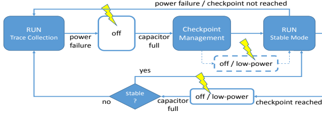
Figure 1. Flow of runtime states
