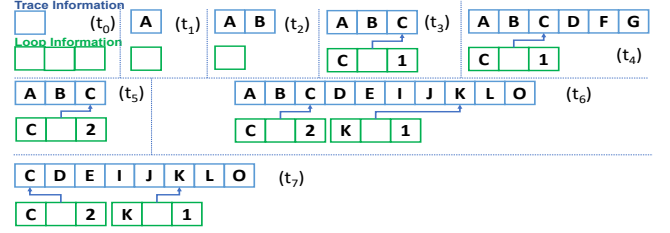
Figure 3. Trace Collection while executing basic blocks
