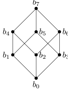
FIGURE 1. The Boolean algebra \mathbf{B}_k for k = 3 .
