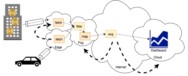
Figure 1. Use case: processing smart building data
