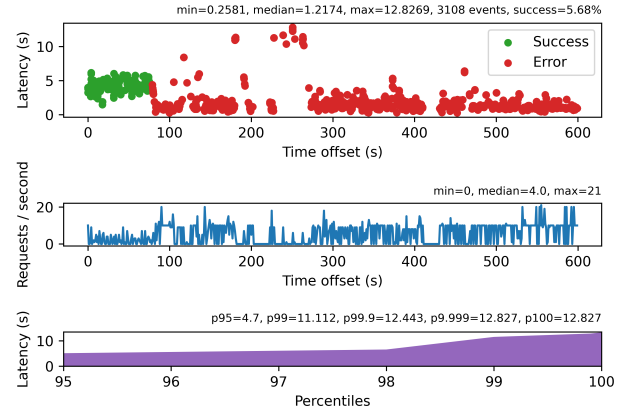
Figure 8. OpenFaaS behavior with 10 workers
