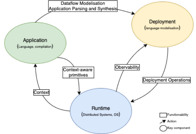
Figure 2. Dyninka Contributions
