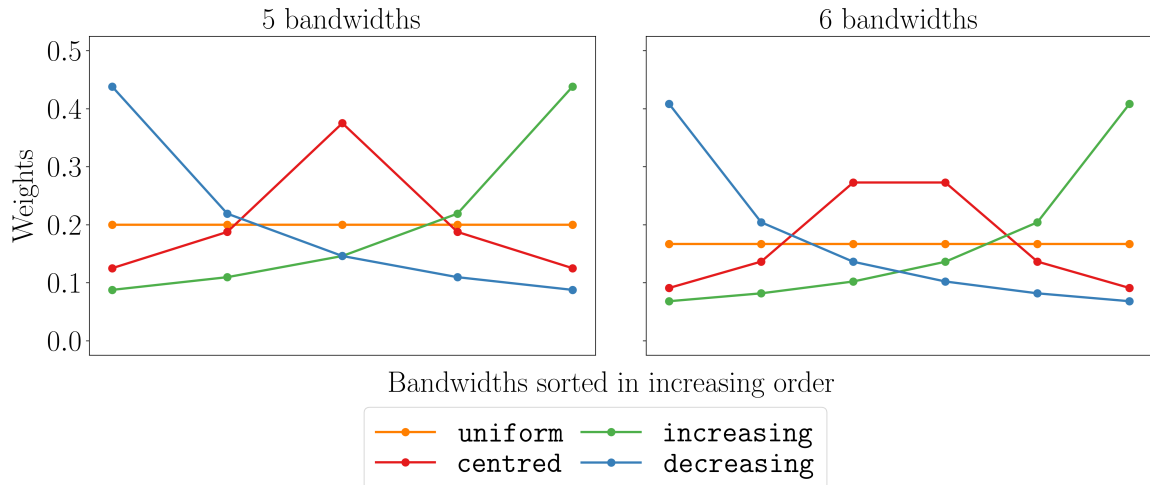
Figure 1: Weighting strategies.
