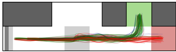
Fig. 3 Traces of 120 replay trajectories for the complex task, with parameters \theta_\tau = 0.3 , \theta_I = 10^{-8} , and \alpha = 0.01 . The colour indicates the target room. Full lines are successful runs, dashed lines are failed runs. Blue lines are runs with collisions.
