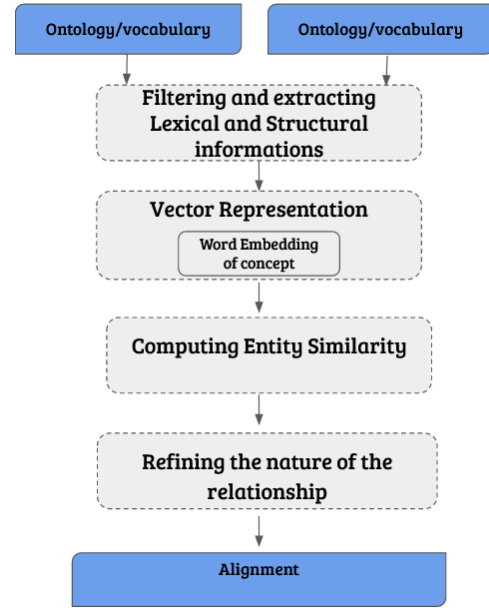
Fig. 1 Workflow of the proposed ontology alignment approach.
