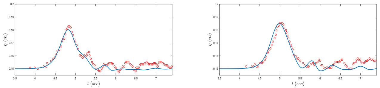
Figure 20: Free surface elevation at wave gauges 3 and 4
