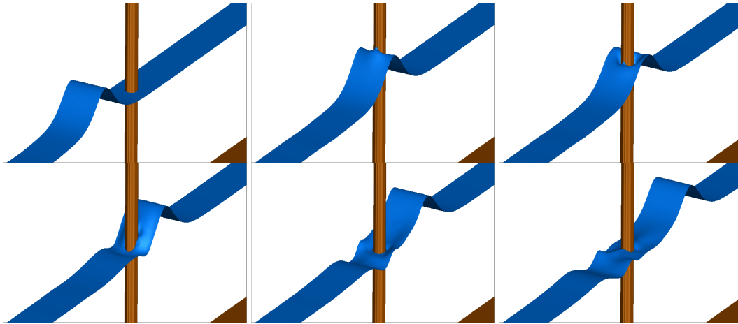
Figure 18: 3D view of the free surface elevation. Interaction of the solitary wave with the vertical cylinder.
