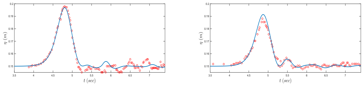
Figure 19: Free surface elevation at wave gauges 1 and 2
