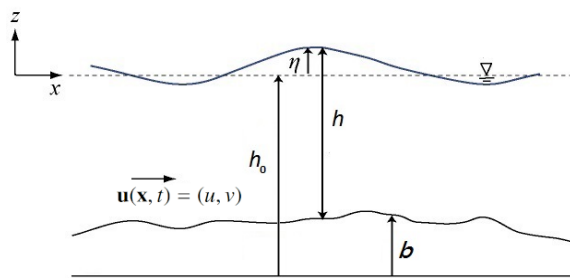
Figure 1: Description of the free surface flow problem and main notation.
