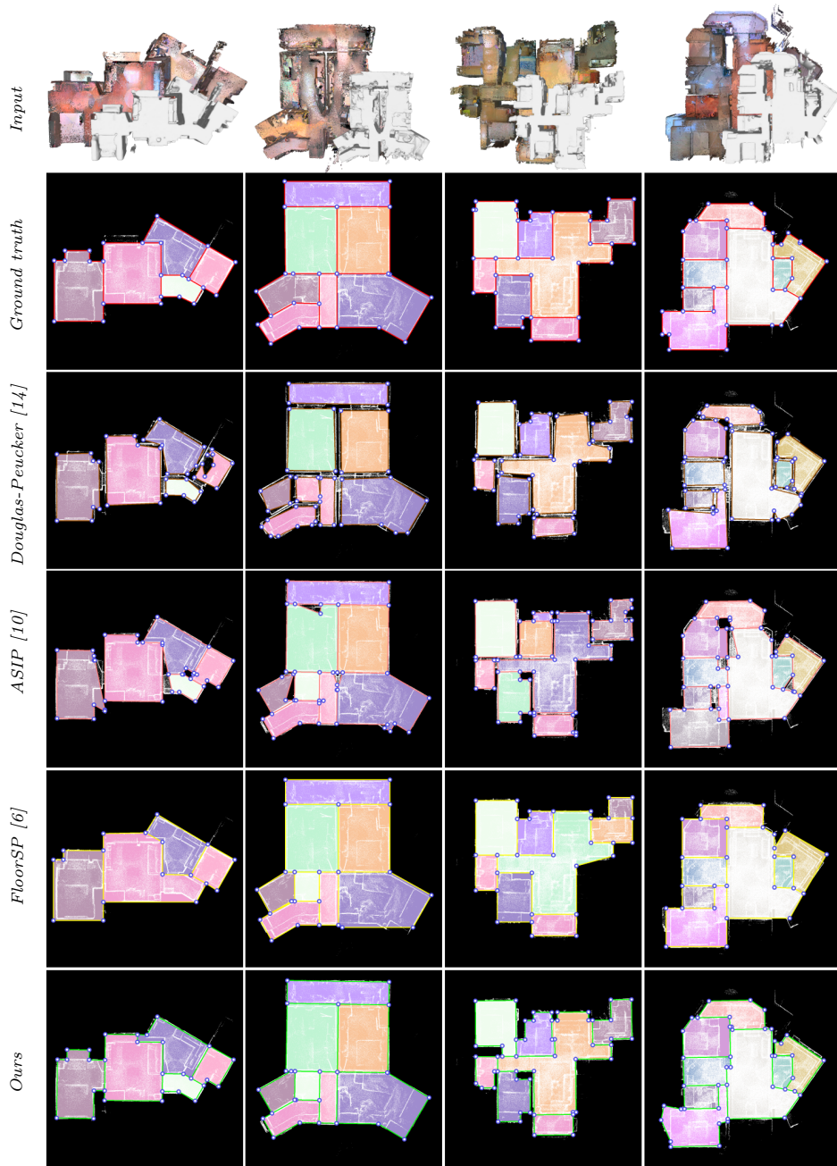
Figure 6: Qualitative comparisons on RGBD scenes. Douglas-Peucker and ASIP return a set of isolated facets while FloorSP and our method produce a valid connected graph. In term of geometric accuracy, floorplans of ASIP and our approach align better with input points than FloorSP and Douglas-Peucker, especially in case of non-Manhattan scenes. In particular, our method achieves to preserve small structure details.
