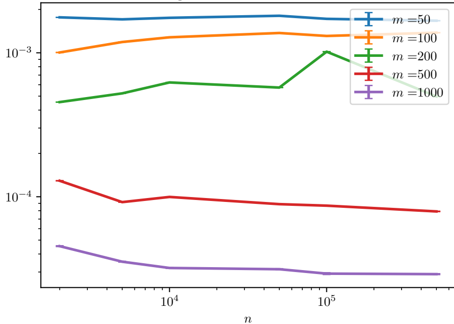
Hellinger distance, d = 10
