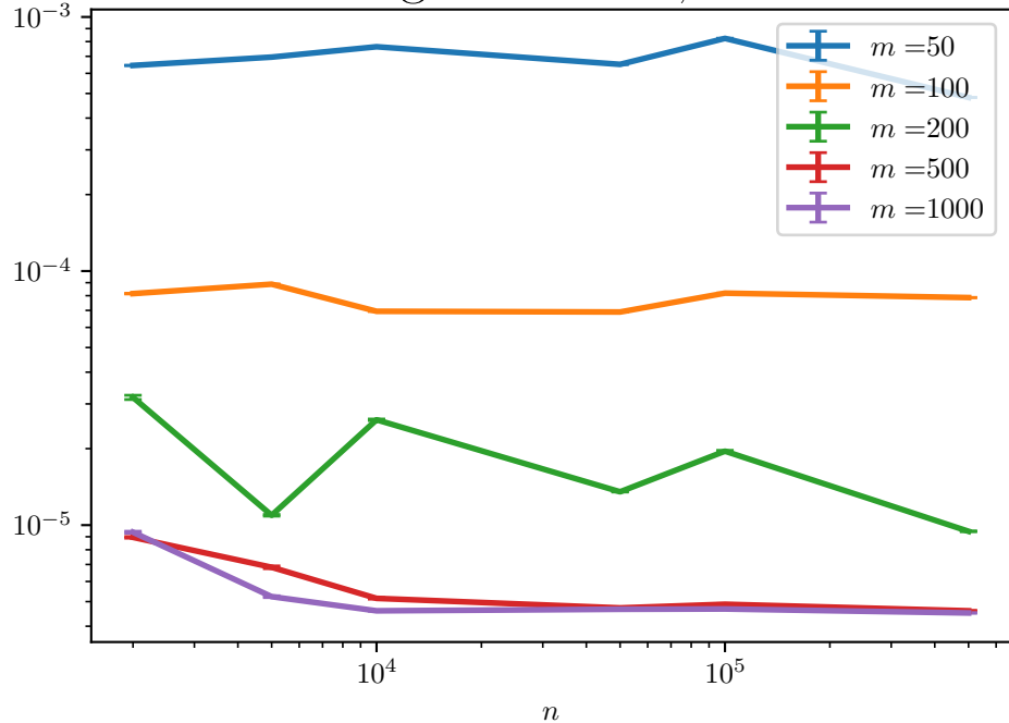
Hellinger distance, d = 2
