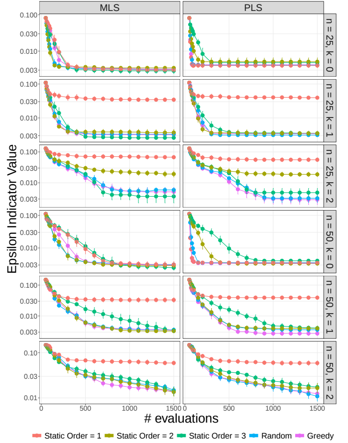
Figure 3. Convergence profile of S-MCO when using different Walsh order settings with the \text{Select}_{B_{\text{norm}}} strategy on MNK-landscapes.
