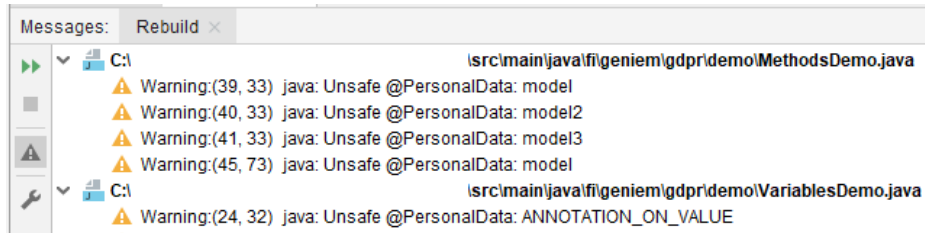
Fig. 3. Example of warnings produced by the analysis in IntelliJ IDEA .
