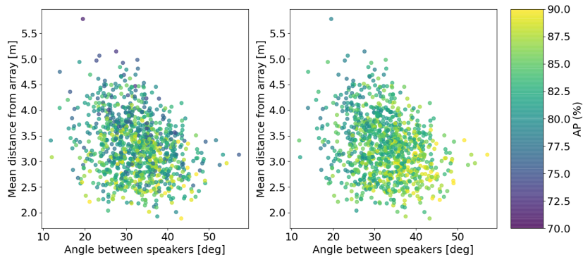
Figure 5: OSD AP (%) achieved on the synthetic evaluation set by the Transformer-based architecture trained with a speaker counting objective as a function of the mean distance of the speakers from the array and the angle between the speakers. Left: single-channel features only. Right: CSIPD spatial features and late fusion.
