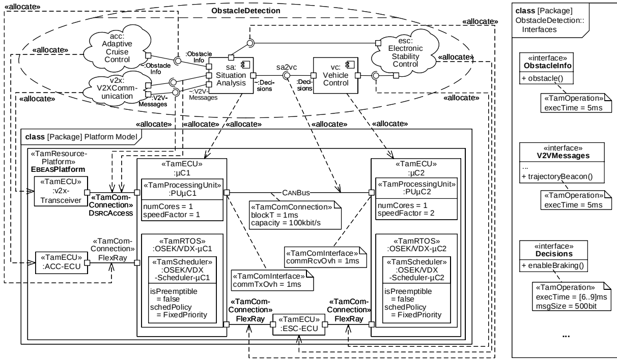
Fig. 7 Platform-specific MSD specification excerpt for the EBEAS
