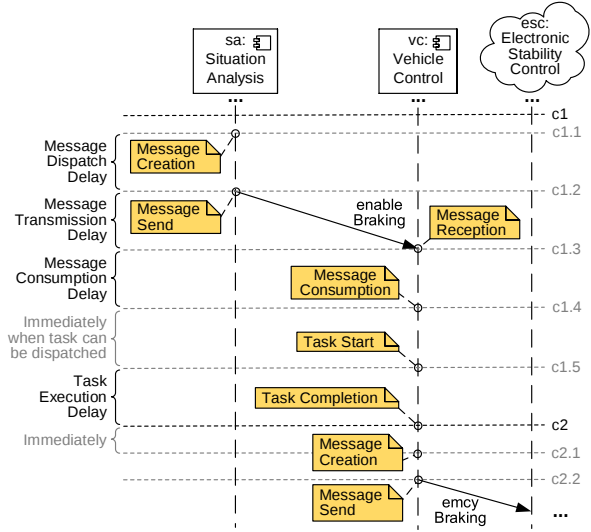
Fig. 9 Additional lifeline location kinds for MSD messages
