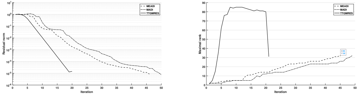
FIGURE 2 TTGMRES, MEADI, and MADI residual histories and maximum TT-rank histories for the cookies problem. The maximum TT-rank of the final approximated solution is appended to the maximum TT-ranks for each method.
