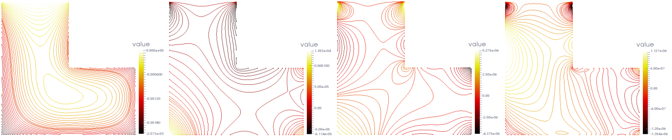
FIGURE 4 First four fibers of the TT-core associated to the space variable, reconstructed by using the finite element space, for the test-case presented in Section 4.2. Contour plots with 40 values between the minimum and the maximum.
