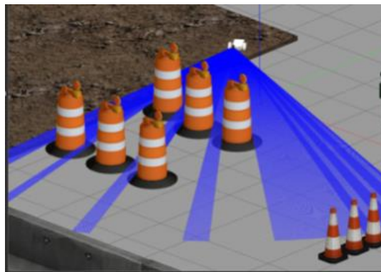
Fig. 3. Example of Sensor (LIDAR) model - Global view
