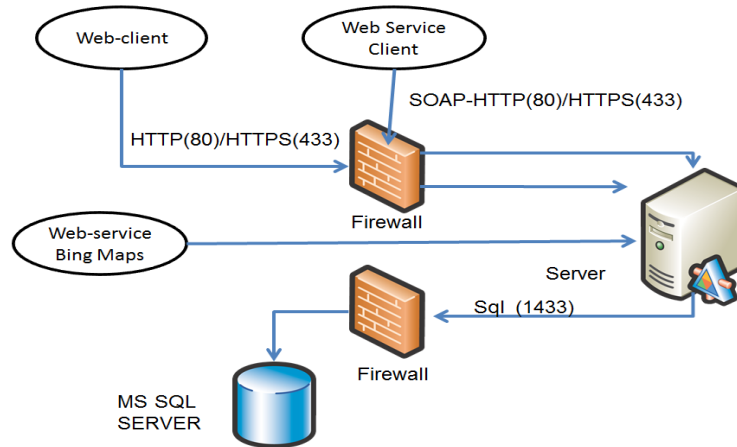
Fig. 5. The EcoSpotter system architecture.
