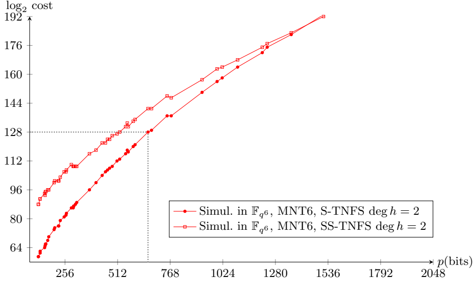
Fig. 8. Estimated cost of DL computation with TNFS in \text{GF}(p^6) .
