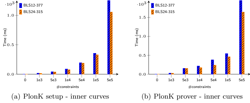
Fig. 4. PlonK Setup (a) and Prove (b) times per number of constraints for inner curves.
