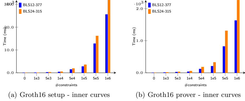
Fig. 3. Groth16 Setup (a) and Prove (b) times per number of constraints for inner curves.
