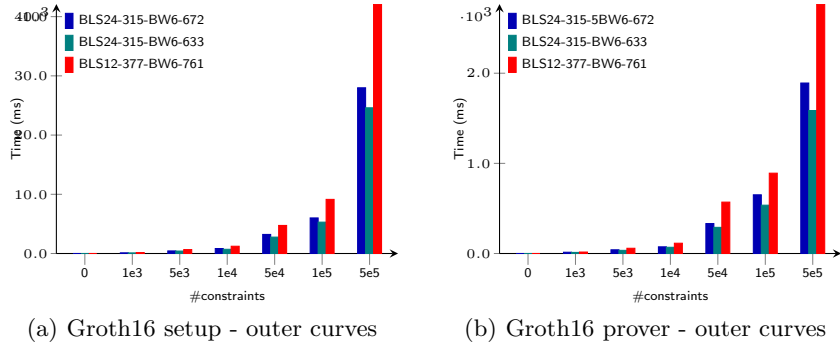
Fig. 5. Groth16 Setup (a) and Prove (b) times per number of constraints for outer curves.
