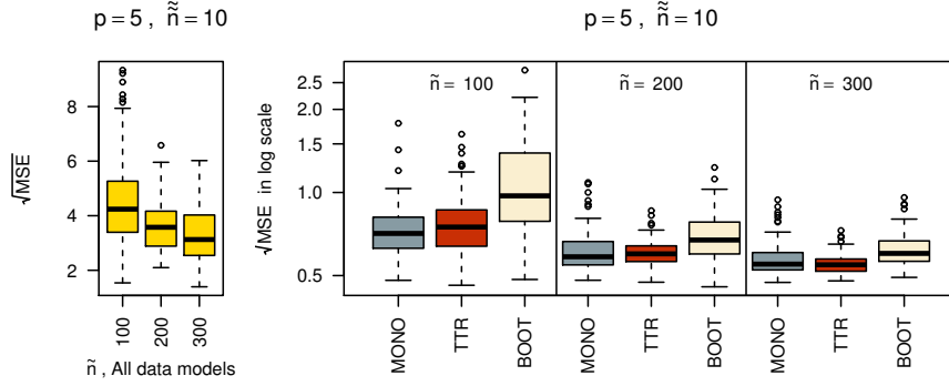
Fig. 6 Root MSE for the different methods. Visualizations of the errors for the complete dataset model (in yellow) and for the three outlier detection methods have been split in two graphics since scales are different. Here p = 5 and \tilde{n} = 10 have been detailed.
