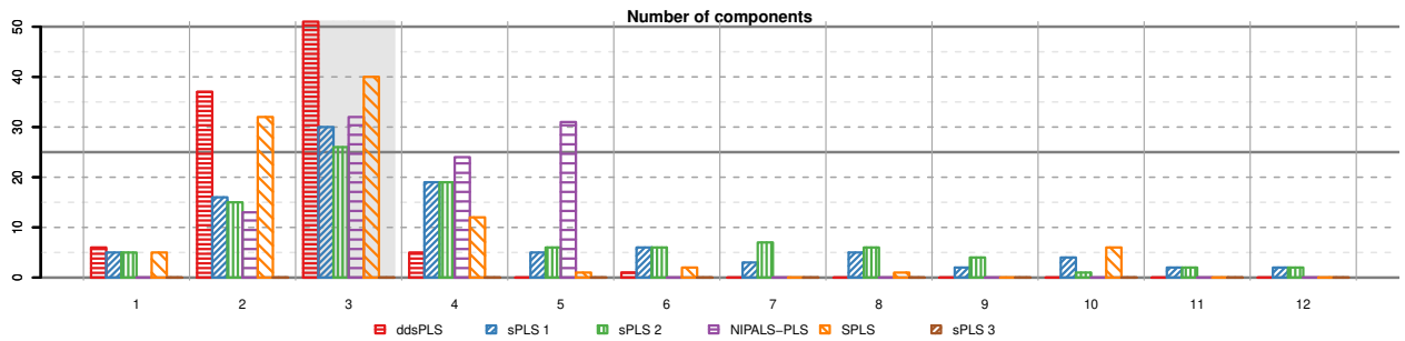
(a) Number \hat{R} of components built for each methodology for design 2. Gray area corresponds to the correct value R = 3 .
