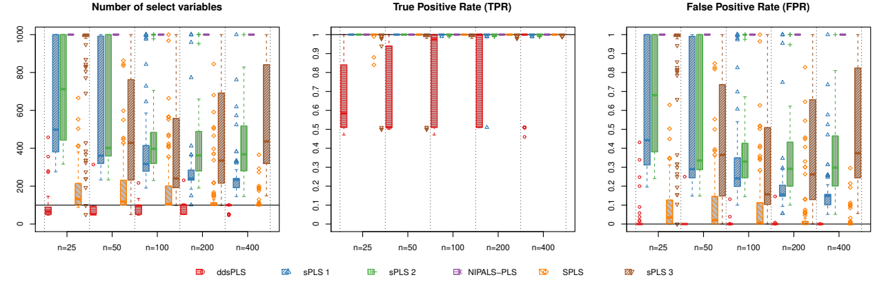
(a) Variable selection performances in the x part.
