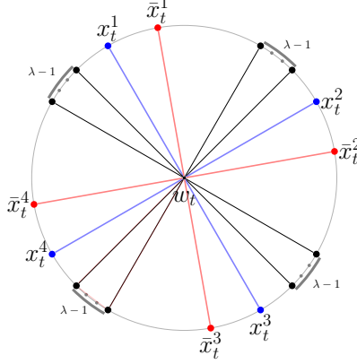
Figure 5: The variable gadget H_t . The center vertex w_t is in a (2\lambda - 1) -degree-gadget. There are four sets of \lambda - 1 vertices (in black) adjacent to the center vertex w_t ; each of them is in a 4\lambda -degree-gadget. Blue and red vertices are respectively non-negated and negated literal vertices. All blue ones (resp. red ones) are adjacent to w_t if and only if \phi(x_t) = \text{true} (resp. \text{false} ).
