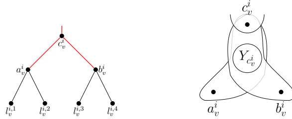
Figure 8: The binary tree T_v^i and an example of the edge-gadget at vertex c_v^i (corresponding to red edges).
