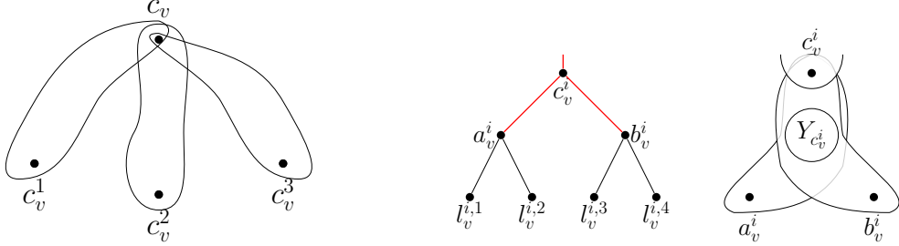
Figure 3: The construction in the reduction. The vertex gadget VG_v in the left with 3 hyperedges (left) in which at least one of c_v^1, c_v^2, c_v^3 can be a (p-1) -vertex in its parent hyperedge. At each of c_v^i , we add to binary tree (middle) where every couple of red edges are replaced by an x -edge-gadget (right) which enforces vertex children having the same degree as its vertex parent in their parent hyperedges. A vertex c_v^i is a (p-1) -vertex in its parent hyperedge S_v^i if and only if v has color i in a proper coloring.
