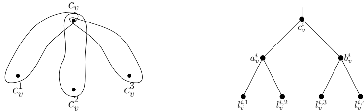
Figure 7: The construction of the reduction. The vertex gadget for vertex v (left) and the color gadget represented as a binary tree with 4 leaves (right). In the construction, each edge of this tree is replaced by hyperedges such that the degree of the root c_v^i is transmitted to all its descendants.
