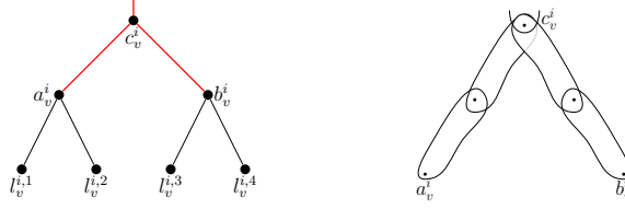
Figure 9: The binary tree T_v^i and an example of the edge-gadget at vertex c_v^i (corresponding to red edges).
