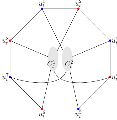
Figure 6: The variable gadget H_t of variable x_t . Blue and red vertices are respectively non-negated and negated literal vertices.
