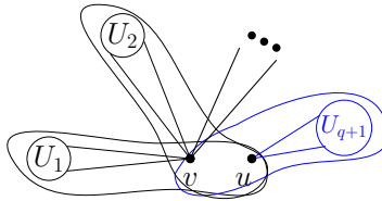
Figure 2: The gadget H_u at vertex u . An example of an (F, H_u, k) -graph where v has degree p - 1 in each of hyperedges U_1, \dots, U_q and u has degree p - 1 in U_{q+1} .
