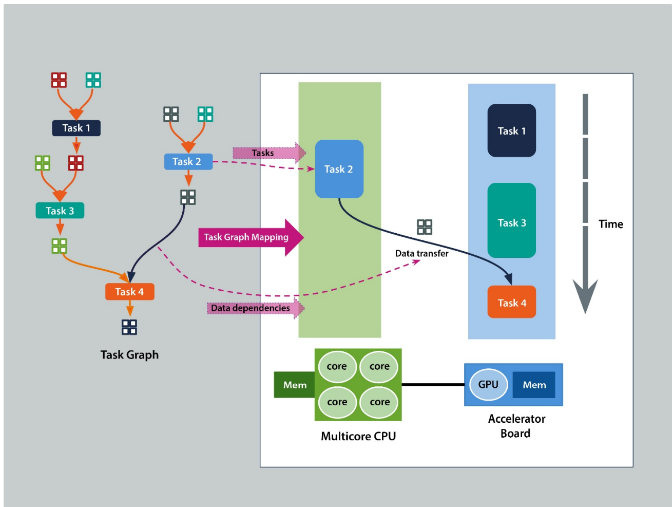
Fig. 2: Illustration of the way the abstract representation of an application given by the task graph can be used by a runtime system to map tasks on available, possibly heterogeneous platforms. Tasks can be dynamically mapped to appropriate processing units using scheduling algorithms. Data consistency between devices can be enforced using data dependence edges. Prefetch operations can be triggered automatically to overlap data transfers with computation.
