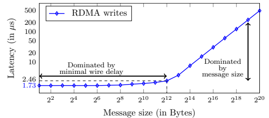
Figure 1: RDMA latency vs data size. Latency remains almost constant up to 4KB message size.
