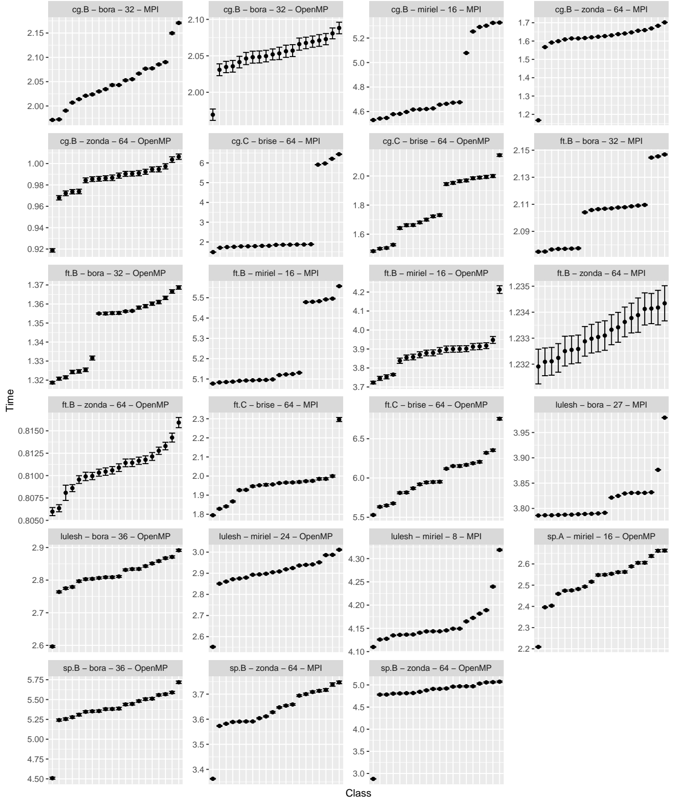
Fig. 2: Comparison of average execution times of mapping classes for different workloads, machines, and programming models.
