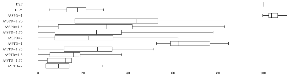
(b) Runtime (in % of the runtime of the DSP Algorithm). A percentage lower than 100 corresponds to a gain of runtime compared to the DSP method.
