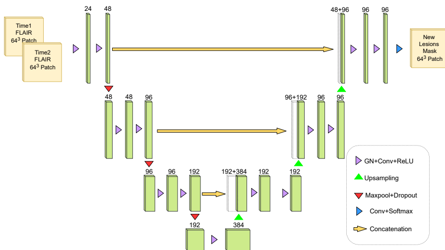
Fig. 1. Illustration of the used U-Net architecture. Each block is composed of group normalization (GN), Convolution (Conv) and Rectified Linear Unit (ReLU) activation.
