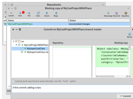
Figure 5-16 When you commit changes, Iceberg shows you the code about to be committed and you can choose the code entities that will effectively be saved.
