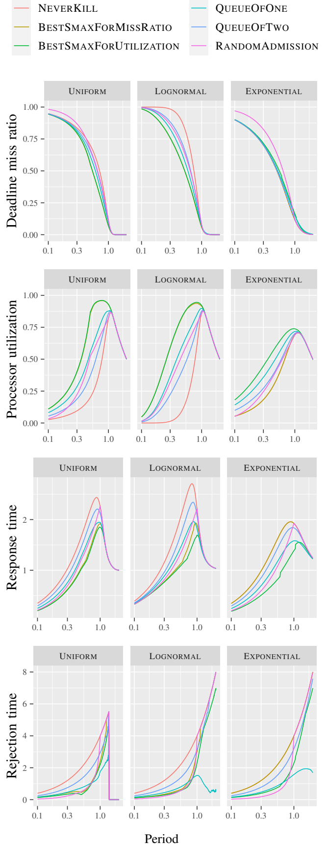
Fig. 1. Performance of the different heuristics.
