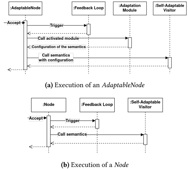
Figure 2. Sequence diagrams representing components interactions when executing a node semantics
