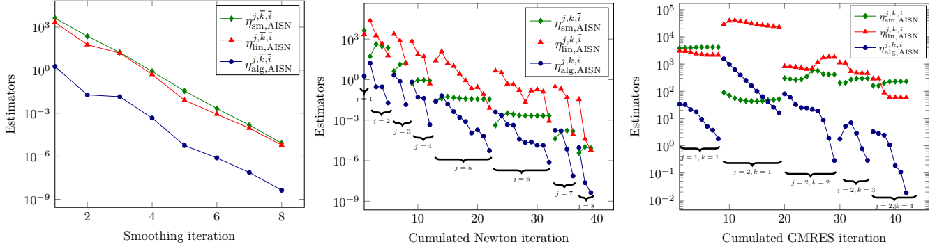
Figure 7: [Adaptive inexact smoothing Newton method, smoothed F–B function (3.2), Algorithm 1] Estimators (3.10) as a function of smoothing iterations j at convergence of the algebraic and linearization solvers, left. Estimators as a function of cumulated Newton iterations at convergence of the algebraic solver, middle. Estimators as a function of cumulated GMRES iterations during the first two smoothing iterations ( j = 1 and j = 2 ), right.
