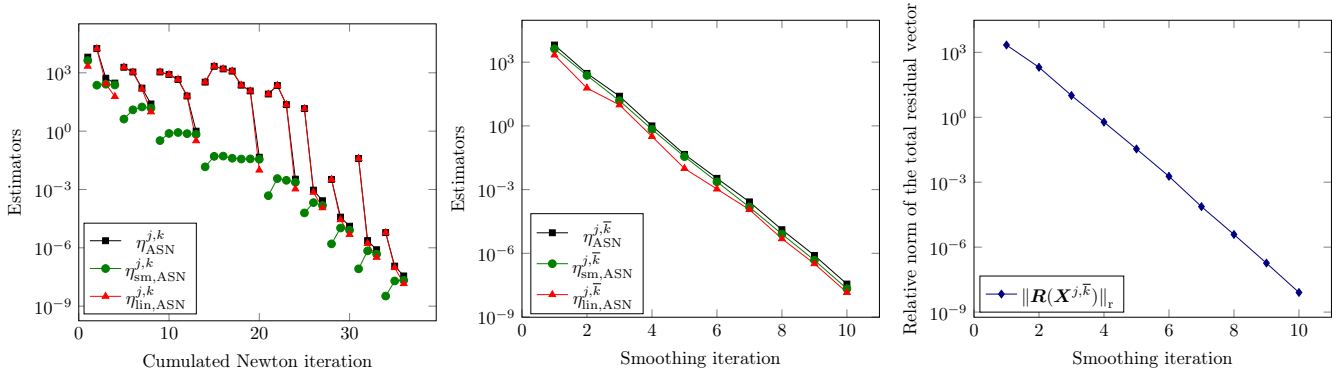
Figure 4: [Adaptive smoothing Newton method, smoothed F–B function (3.2), adaptive stopping criterion (6.5)] Estimators (6.3) as a function of cumulated Newton iterations (left). Estimators (6.3) (middle) and relative norm of the total residual vector (2.6) (right) as a function of smoothing iterations j at convergence of the linearization solver.
