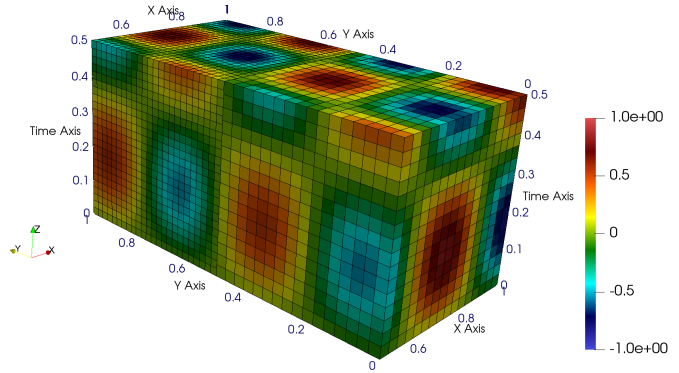
(c) On \Omega_2^T \cup \Omega_3^T
