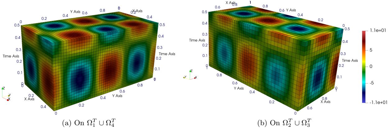
Figure 4: Example 1, y -component of velocity computed using bilinear mortars shown on the space-time grid at refinement 3.
