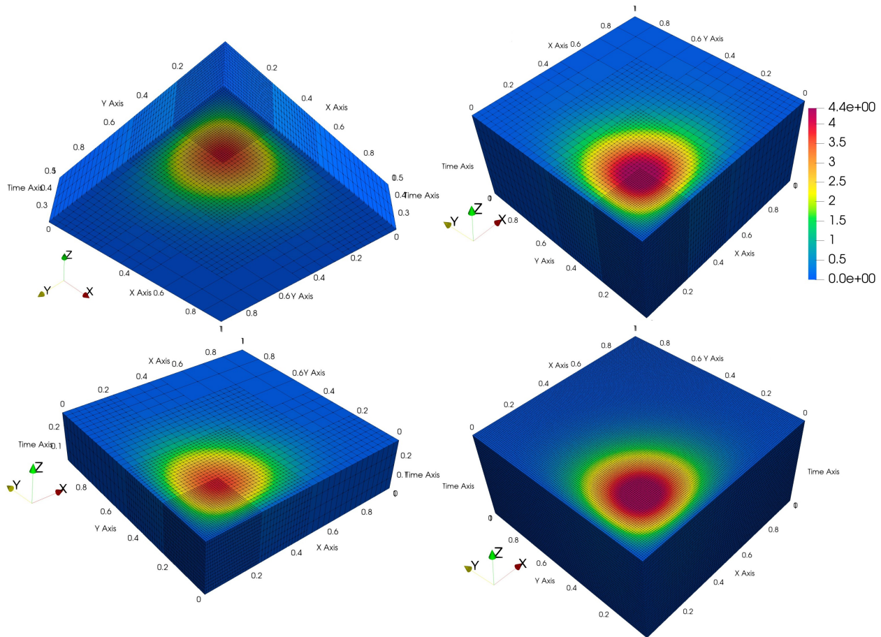
Figure 6: Example 2, left: pressure from the multiscale method, cut along the plane t = 0.35 ; right: pressure from the multiscale (top) and fine-scale (bottom) methods on the whole domain.
