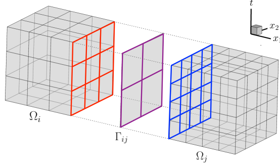
Figure 1: Non-matching space-time subdomain and mortar grids in two spatial dimensions.
