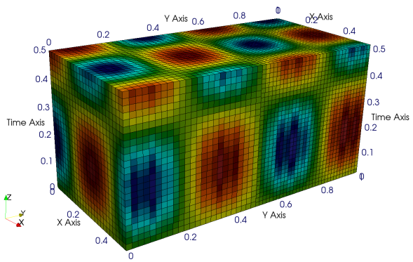
(a) On \Omega_1^T \cup \Omega_4^T
