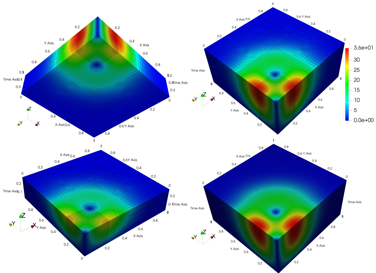
Figure 8: Example 2, left: velocity magnitude from the multiscale method, cut along the plane t = 0.35 ; right: velocity magnitude from the multiscale (top) and fine-scale (bottom) methods on the whole domain.
