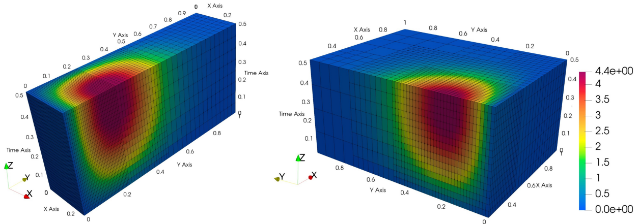
Figure 5: Example 2, pressure from the multiscale method, cut along the plane x = 0.25 .
