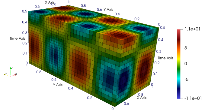
(b) On \Omega_2^T \cup \Omega_3^T
