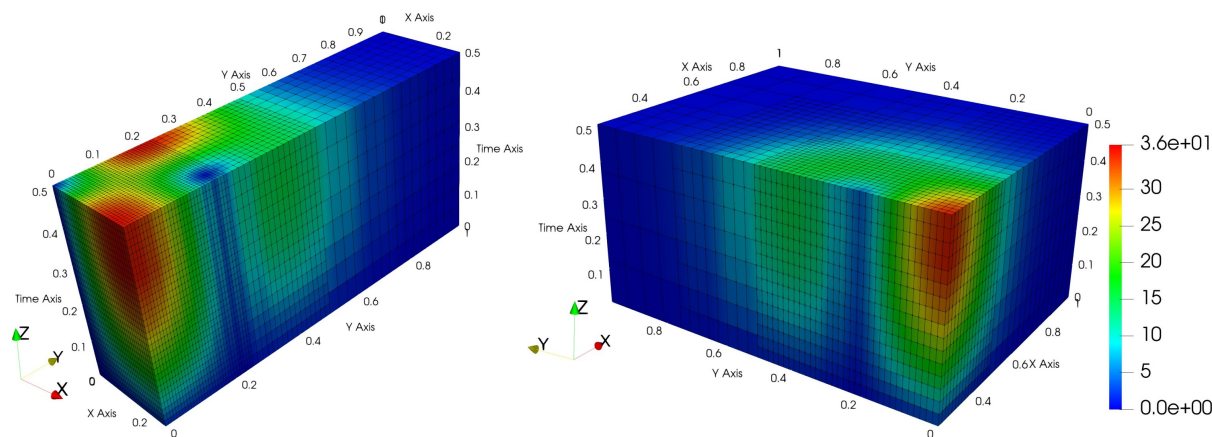
Figure 7: Example 2, velocity magnitude from the multiscale method, cut along the plane x = 0.25 .
